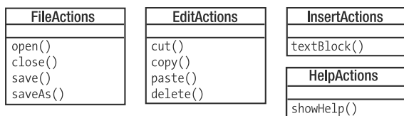
Figure 16-1. The methods supported by the receiver classes
