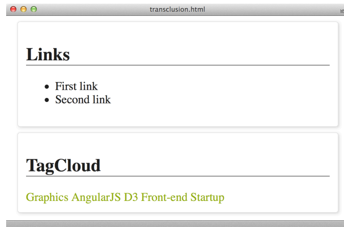
sidebox
