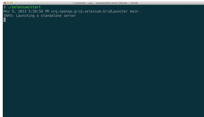
Install Selenium
