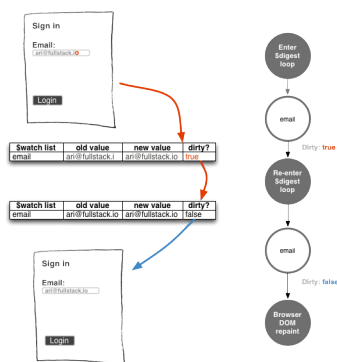
Digest loop
