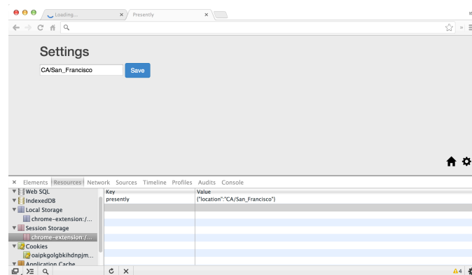
sessionStorage
