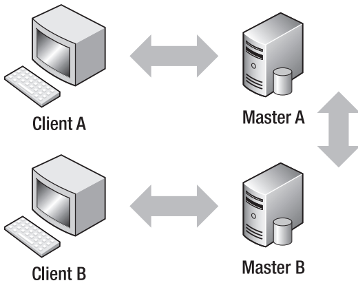
Figure 11–4. Master/master replication
