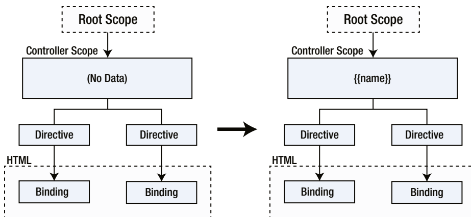
Figure 16-5. Multiple instances of a directive operating on the controller scope
